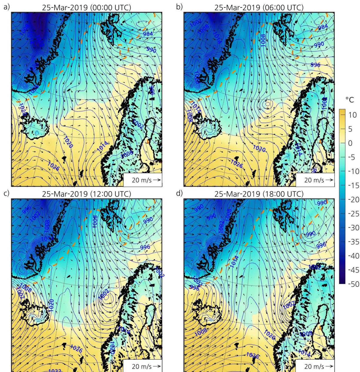
Fig 2. ERA5 atmospheric fields showing the development of the PL on 25 March 2019 at (a) 0000 UTC, (b) 0600 UTC, (c) 1200 UTC, and (d) 1800 UTC. The blue isolines represent the SLP (contours every 2 hPa), the colourmap represents the 2-m temperature ( ^{\circ}\text{C} ), and the arrows represent the 10-m wind direction and speed, with longer arrows representing higher wind speeds. The orange dashed line represents the sea ice edge, which is defined as the 0.15 contour of the SIC corresponding to 25 March 2019 at 1200 UTC. The black outlining represents the coastline. ERA5 fields have been interpolated to the grid of the simulation using bicubic interpolation for the SLP and temperature and bilinear interpolation for the wind. The dataset used to plot the geographic contours has been obtained from the GSHHG [33] under a CC BY license, with permission from Dr. Paul Wessel.
