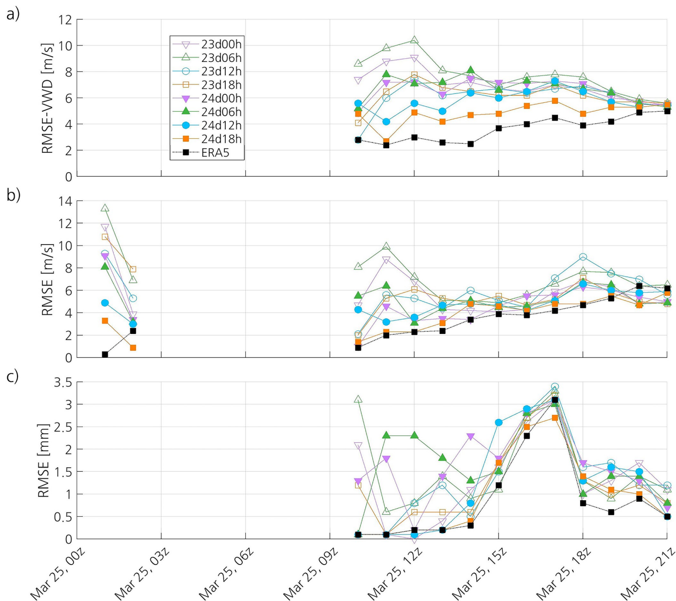
Fig 11. Time series of the (a) RMSE-VWD of the simulated and ERA5 10-m wind, and RMSE of the simulated and ERA5 (b) wind gusts and (c) 1-h accumulated precipitation. The datasets used as reference to compute the RMSE-VWD and RMSE are the observations at surface stations.
