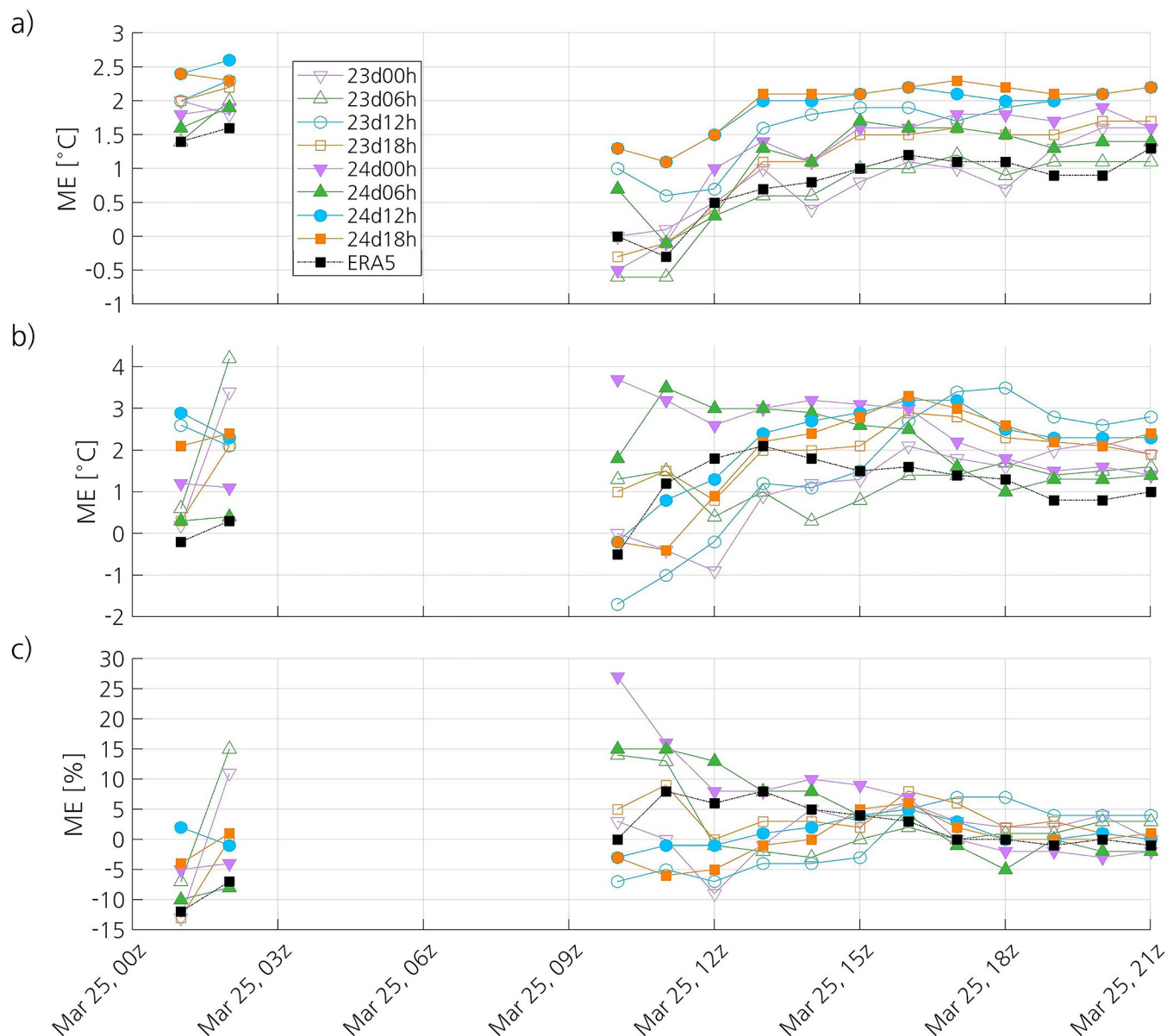
Fig 10. Time series of the ME of the simulated and ERA5 (a) 2-m temperature, (b) 2-m dewpoint temperature and (c) 2-m relative humidity. The datasets used as reference to compute the ME are the observations at surface stations.
