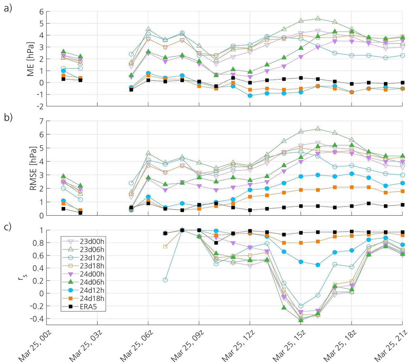
Fig 8. Time series of the (a) ME, (b) RMSE, and (c) Spearman correlation coefficient of the simulated and ERA5 SLP. The dataset used as reference to compute the ME is the SLP measured at surface stations and drifting buoys.
