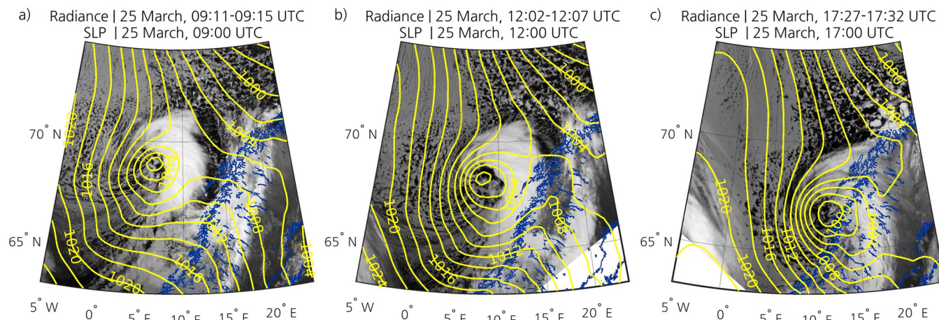
Fig 3. AVHRR channel 4 images showing the PL on 25 March (a) before it hits land, (b) when it is over a great part of the Norwegian coast, and (c) when it starts to dissipate. The yellow isolines represent the ERA5 SLP field (contours every 2 hPa). The blue outlining represents the coastline. The dataset used to plot the geographic contours has been obtained from the GSHHG [33] under a CC BY license, with permission from Dr. Paul Wessel.
